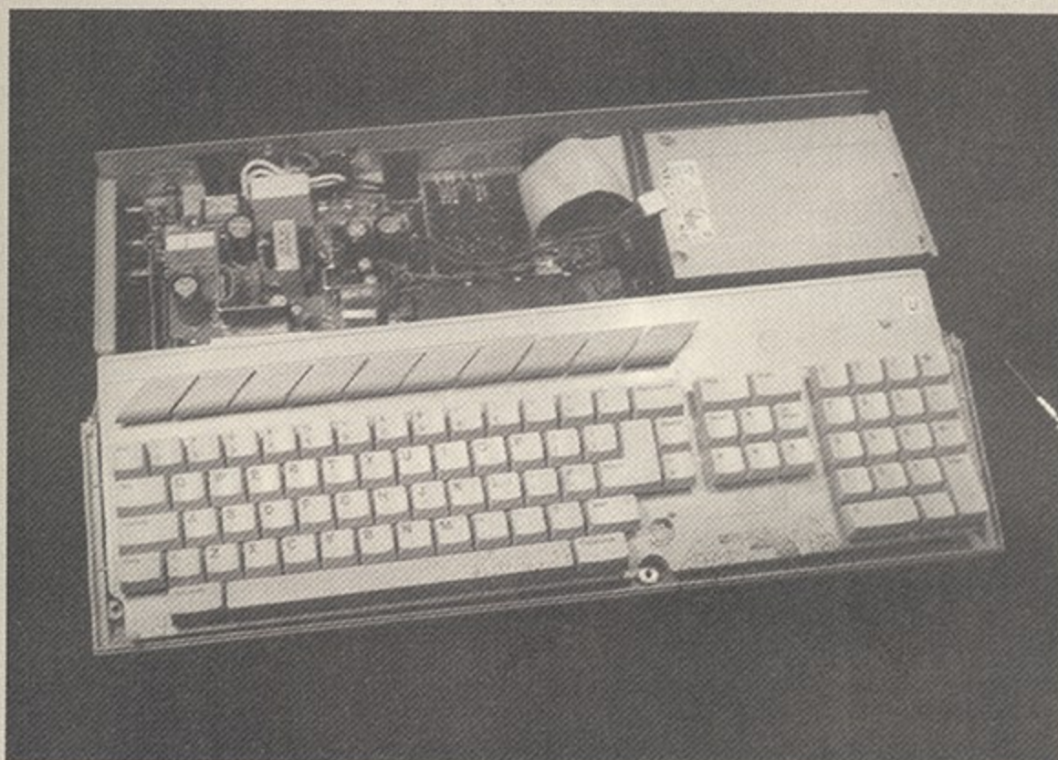
• Pop the new drive into place and reconnect the cables. Now all you have to do is reassemble the ST by reversing the process and you're done.
