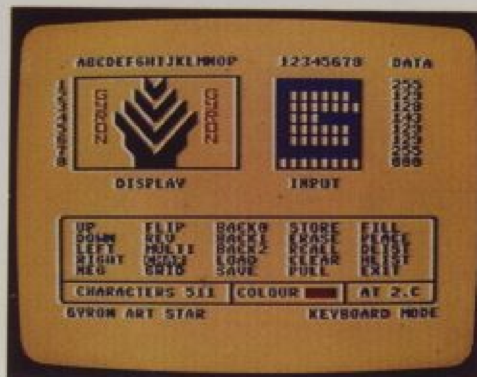
CHARACTER EDITOR
