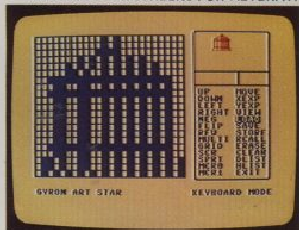
SPRITE EDITOR
