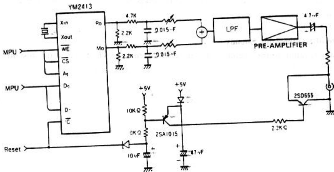
Figure IV - 2 Audio interface
