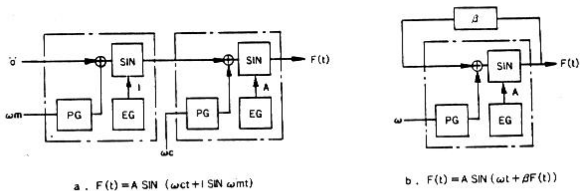
Figure I-1 Sound synthesis by FM with units
