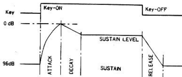
Figure III - 2 Envelope waveform
