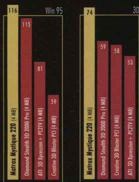
Matrox outperforms the competition (16-bit)
