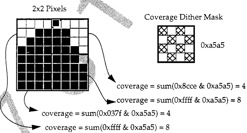
Figure 16-4 Coverage Calculation
