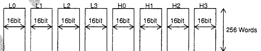
Figure 14-9 Physical Tmem Diagram
