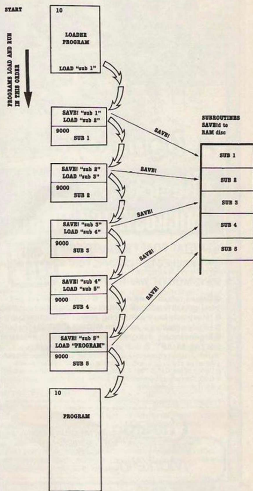
Figure 5. Loading daisy-chained subroutines.
