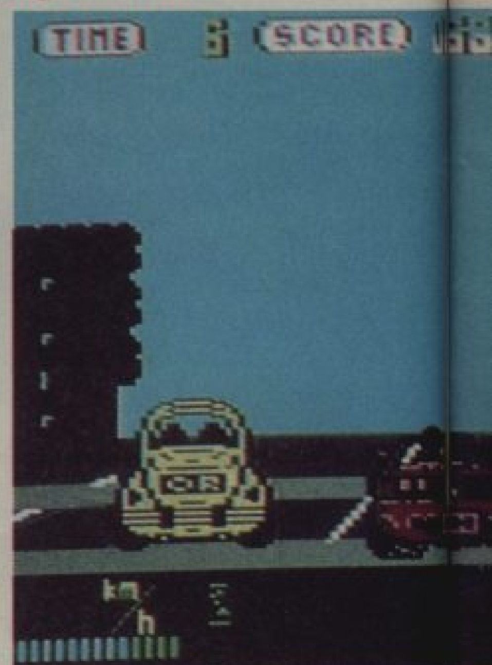
△ COMMODORE 64
