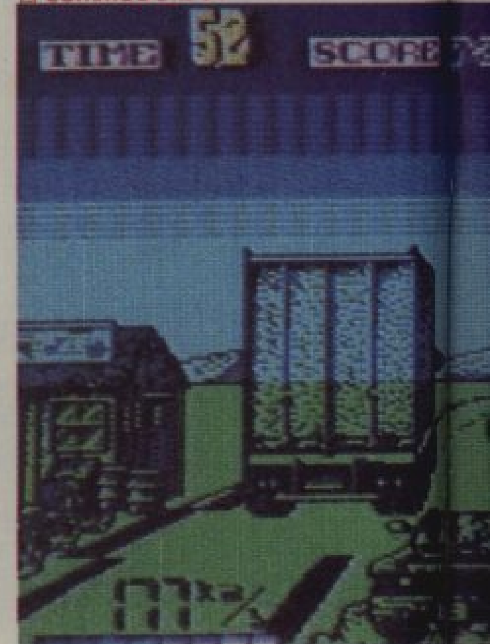
△ COMMODORE 64
