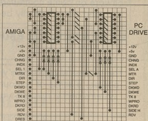
• The stripboard diagram of the circuit.
