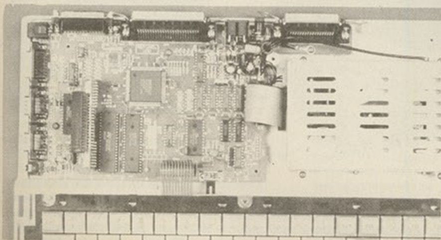
• The guts of a Plus. The new features come from the square chip in the centre of the board.
