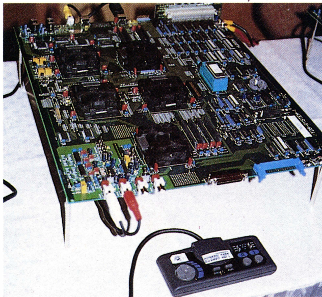
The provisional Tetsujin hardware includes a 25 Mhz RISC processor, and a custom chipset developed by hardware guru Hudson
