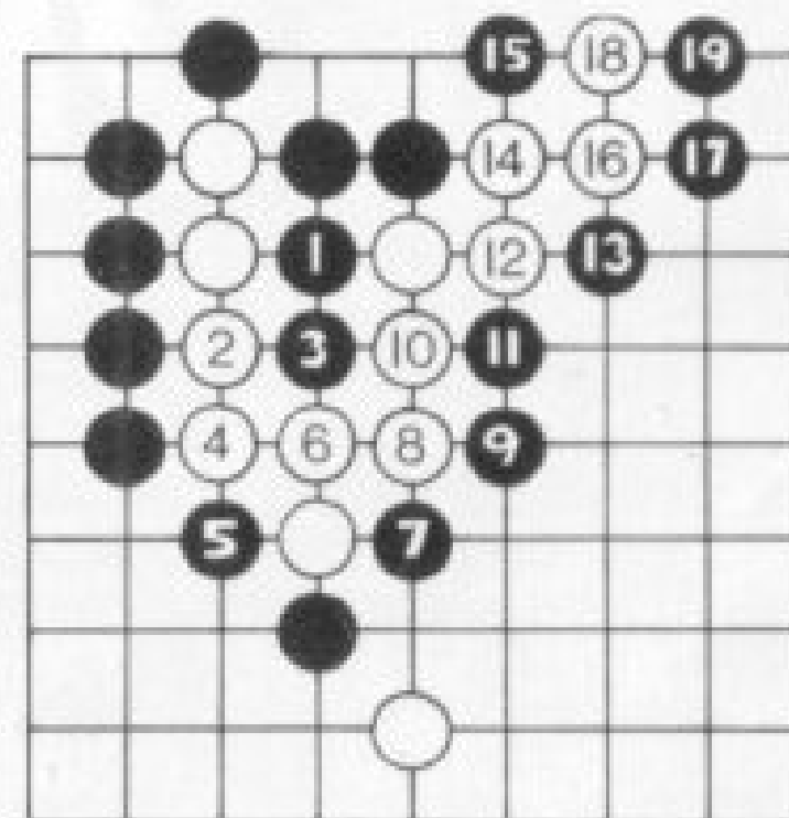
Figure 4: Ladders can bend
