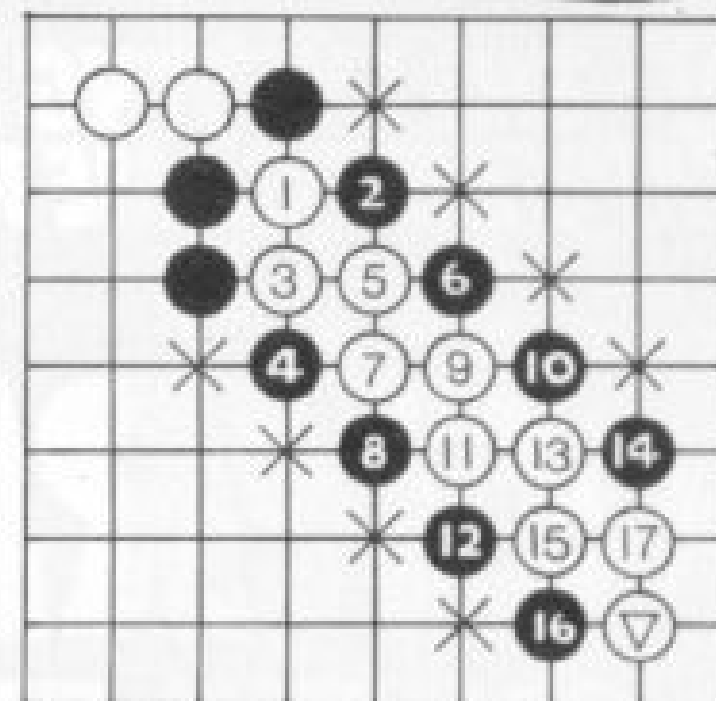
Figure 2: A ladder breaker
