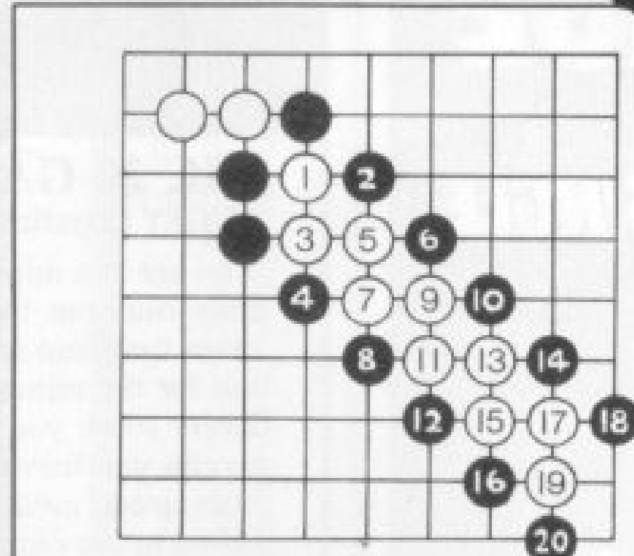
Figure 1: A successful ladder
