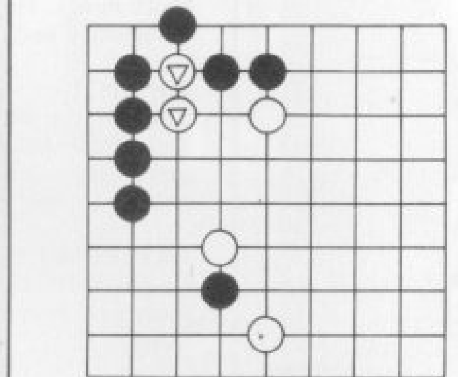
Figure 3: Can white be ladderred?
