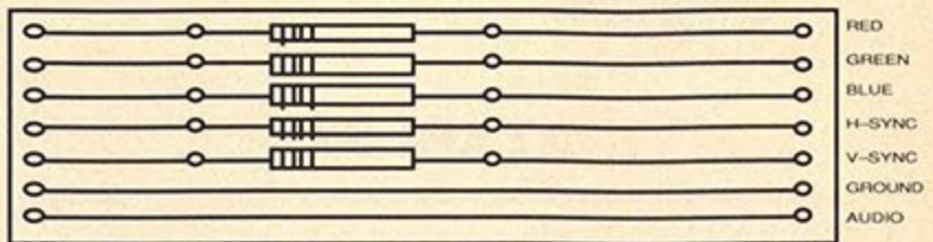
7-PIN DIN SOCKET - INTERNAL CONNECTIONS
