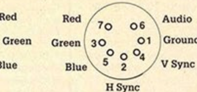
7-PIN DIN PLUG INTERNAL CONNECTIONS
