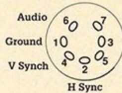
7-PIN DIN SOCKET - INTERNAL CONNECTIONS
