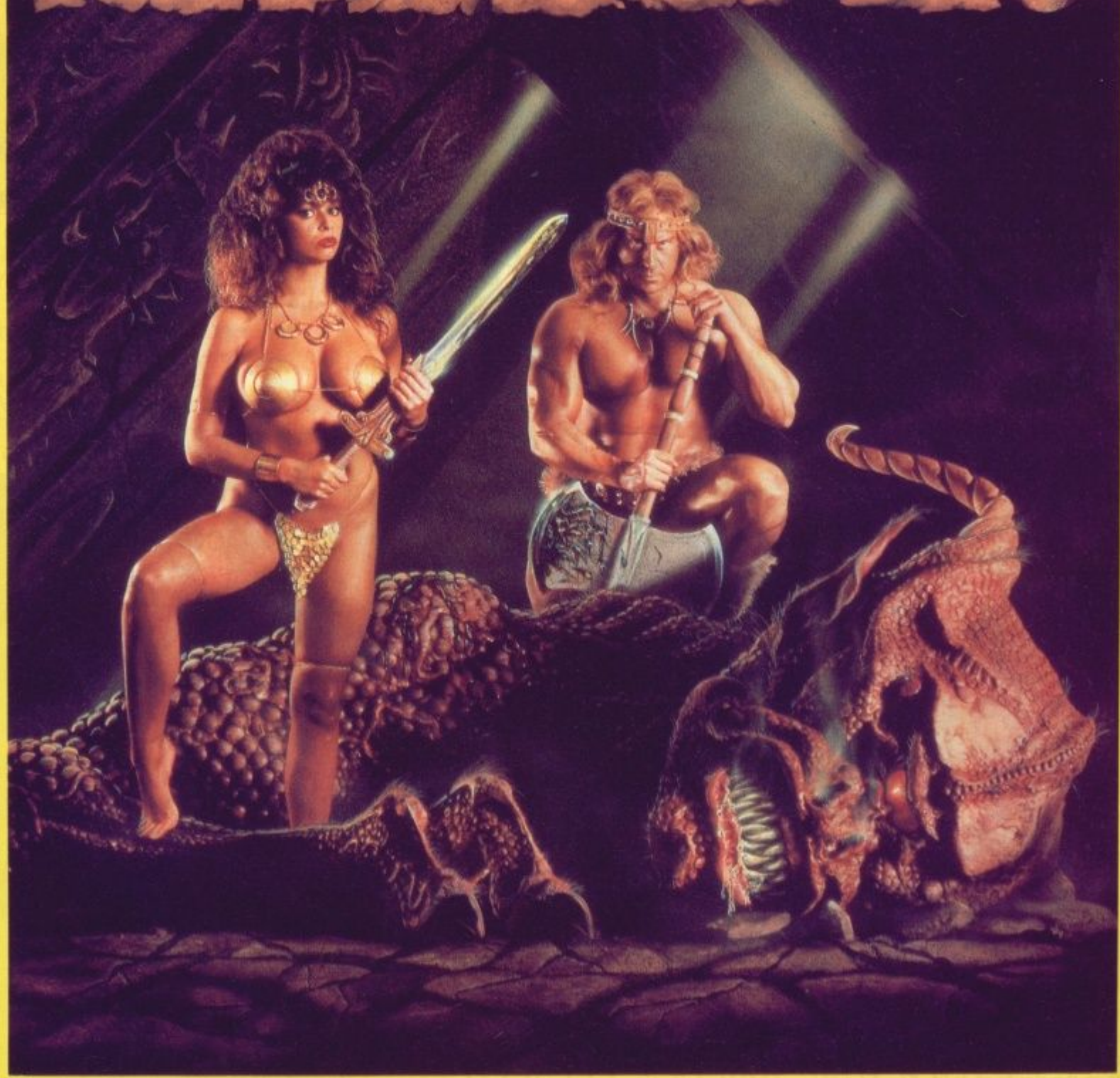
Spectrum Version
