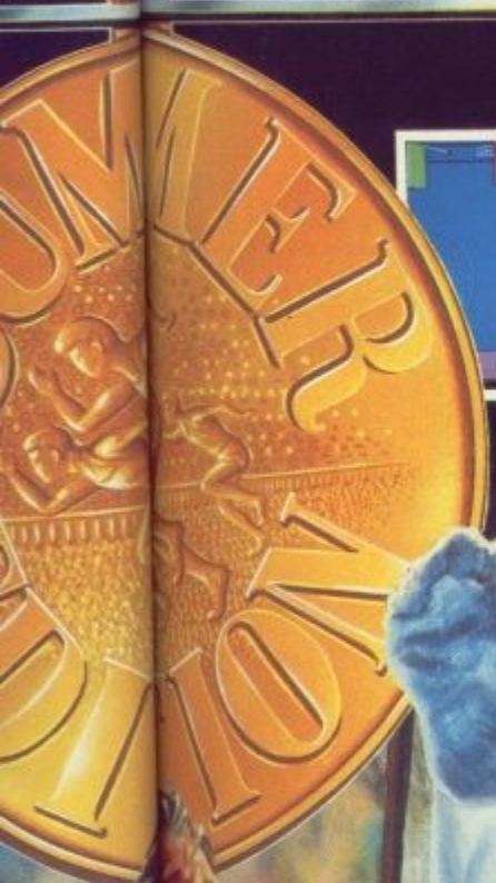
CBM 64
