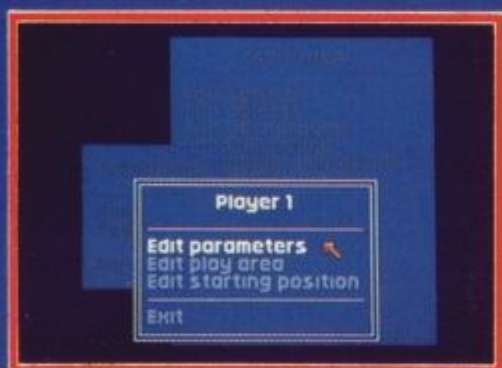
menu driven
