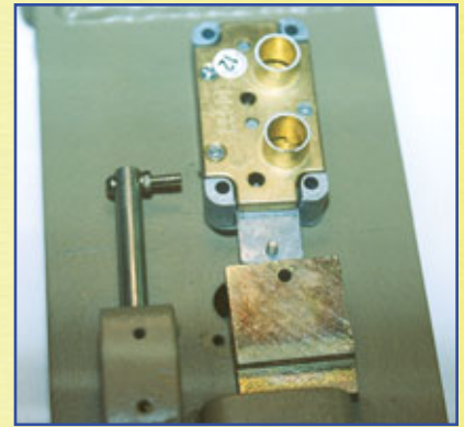
10. ILCO lock with screw at end of long bolt fits into hole of door bolt.
