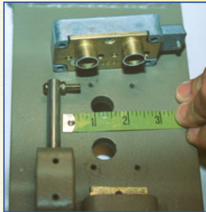
9. Relock bolt position about 1.25 inches below right-handed lock.
