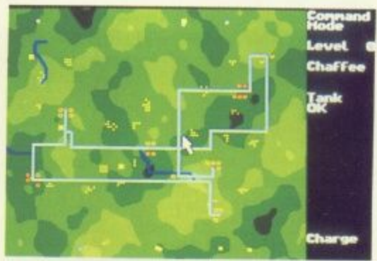
The map shows landscape features and the Yellow and magenta dots denote opposing tanks
