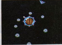
Mercury
