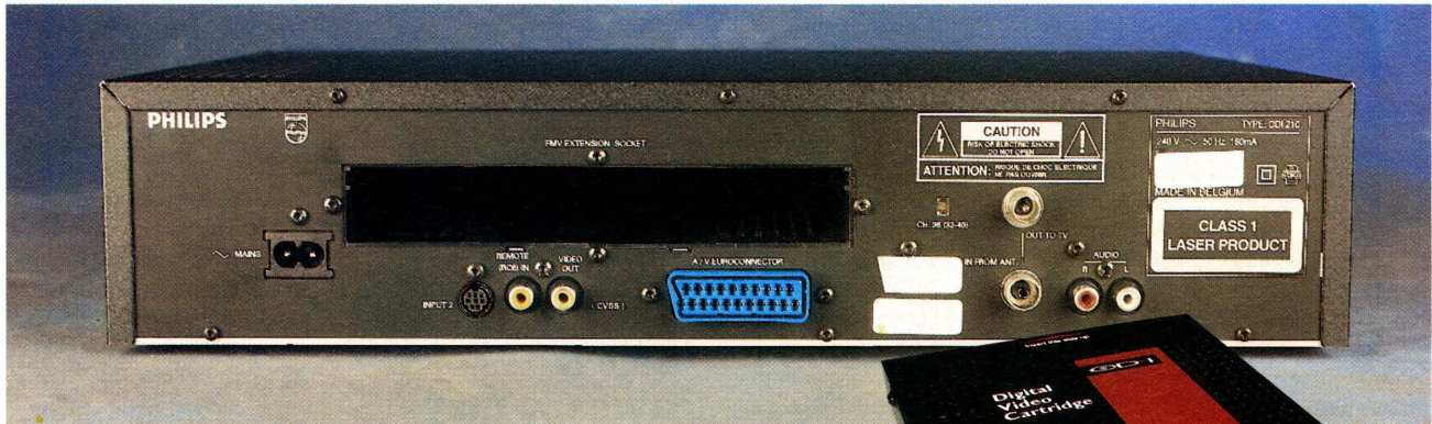
At the rear of the CD-i 210 are: a 21-pin SCART socket, audio and composite video RCA sockets, and the accommodating recess of the FMV port, for connection to the DV cart
