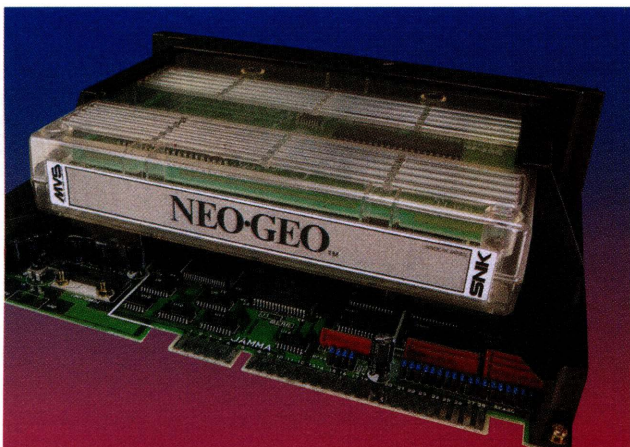
The Neo Geo MV-FZ1 is a single-slot JAMMA-standard PCB that plays Neo Geo MVS arcade cartridges (see letter from Alan Partridge)
