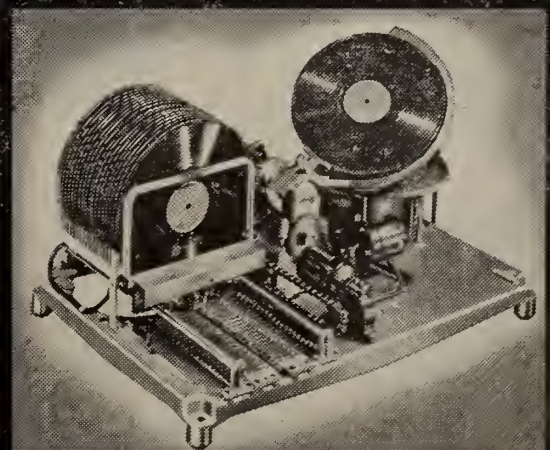
Famous trouble-free AMI changer. 20 records, 40 selections. The one thoroughly field proven mechanism.
