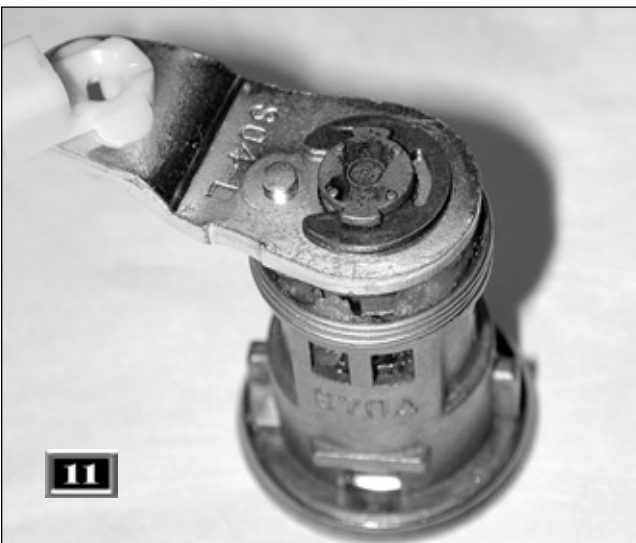
The tailpiece is held on with a common "C" clip. There are no codes on any locks.
