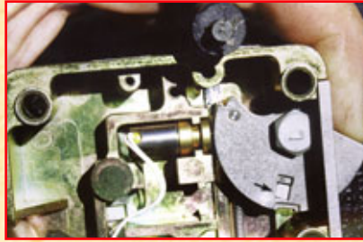
3. Showing the bolt swinging out of the way. Arrow points to the anti-forcing mechanism of the lock bolt itself.
