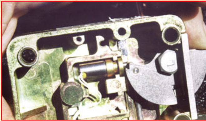
1. Solenoid, pin, and lock swingbolt of the LaGard 3600 electronic lock.
