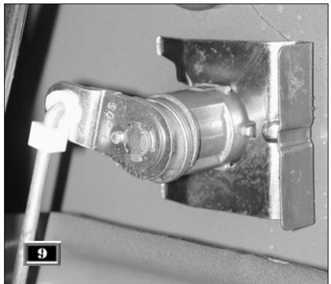
Looking inside the door cavity we see the standard Horse Shoe style metal clip.
