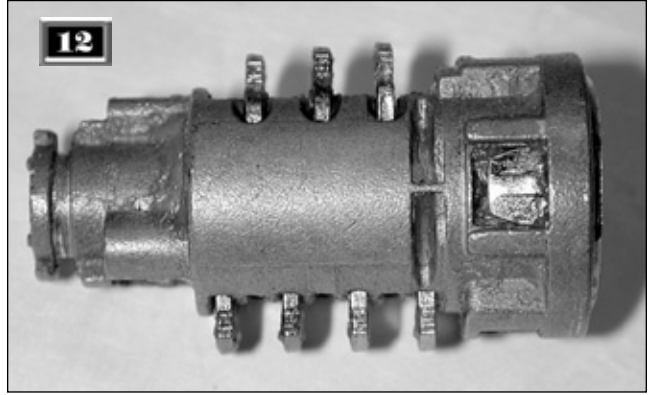
The door lock plug contains 7 tumblers in positions 1 through 7.
