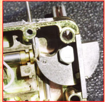
2. Long screwdriver from side of lock case pushing in the solenoid pin allowing the bolt to swing open.
