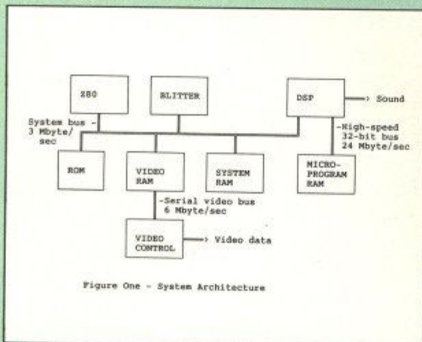
The Flare One's Architecture
